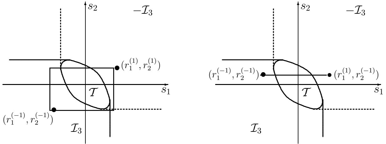
Figure A.1: Intersections of the box \mathcal{R} and \mathcal{T} : (a) the case r_1^{(-1)} \leq r_2^{(-1)} \leq -1 < r_3^{(-1)} \leq 1 , (b) the case r_1^{(-1)} \leq -1 < r_2^{(-1)} \leq r_3^{(-1)} \leq 1
