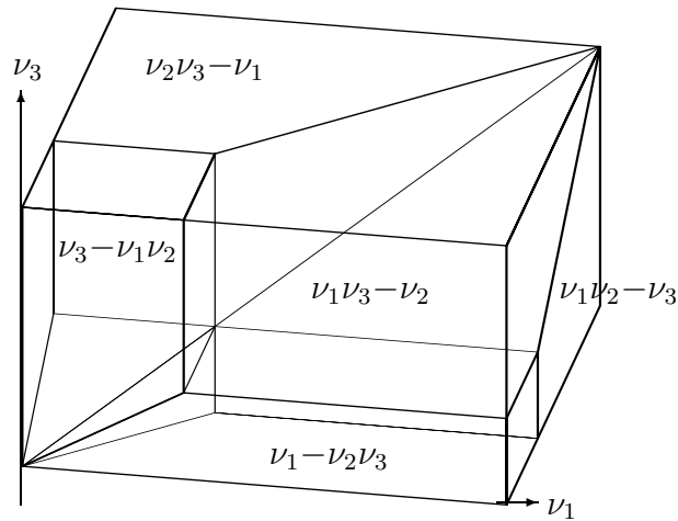
Figure 3.1: The function \Psi : \nu \mapsto \max\{|\nu_1 - \nu_2 \nu_3|, |\nu_2 - \nu_1 \nu_3|, |\nu_3 - \nu_1 \nu_2|\} .
