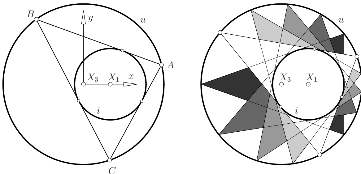
Figure 1: Triangle \Delta with incircle i , circumcircle u , and the Cartesian coordinate system imposed on it
