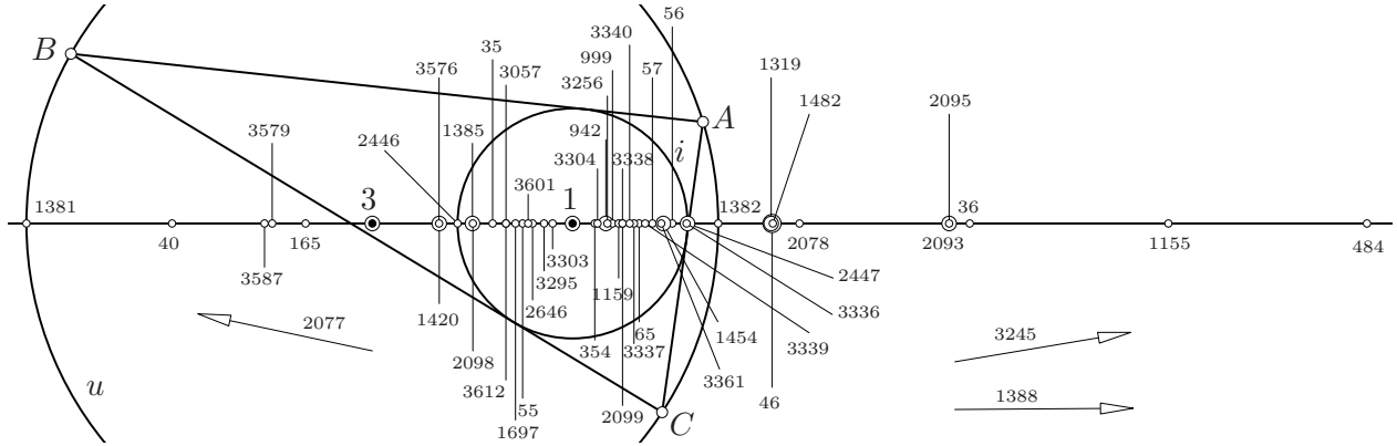
Figure 6: Distribution of fixed centers on \mathcal{L}_{1,3}
