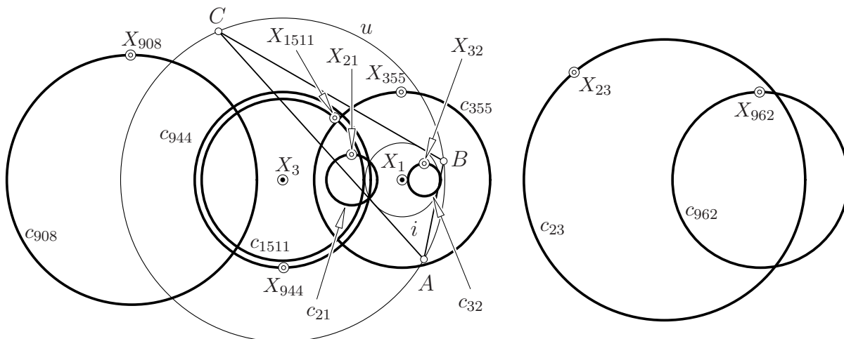
Figure 12: Poristic loci of the SCHIFFLER point X_{21} , the Far-Out point X_{23} , the 3 rd power point X_{32} , the FUHRMANN center X_{355} , the point ACUBENS X_{908} , the HOFSTADTER-TRAPEZOID point X_{944} , the LONGUET-HIGGINS point X_{962} , and the FERMAT crosssum X_{1511} .
