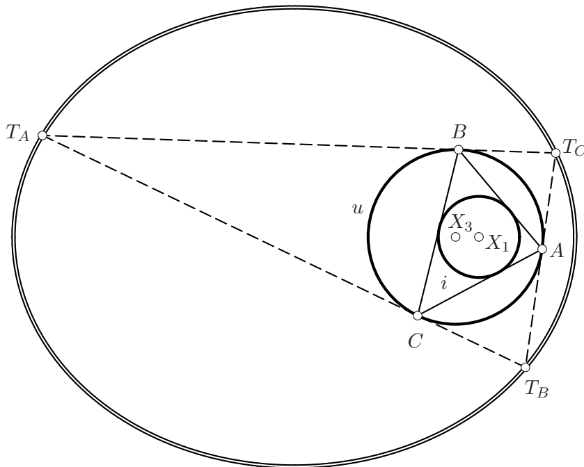
Figure 4: The ellipse traced by the vertices of the tangential triangle.
