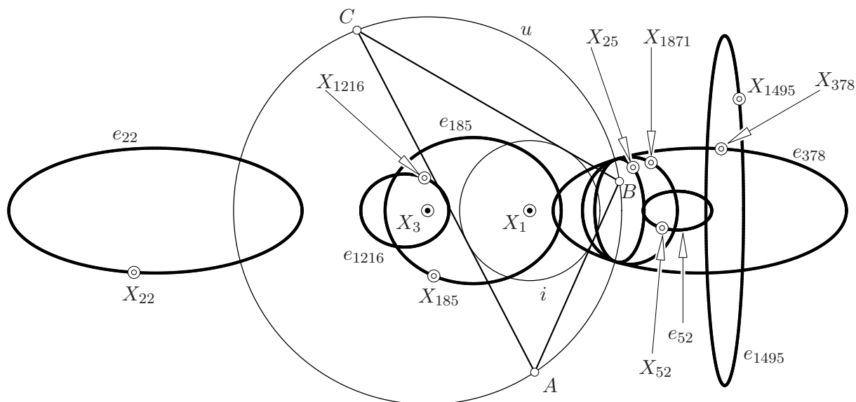
Figure 13: Some ellipses being poristic loci of triangles, cf. Theorem 4.7.
