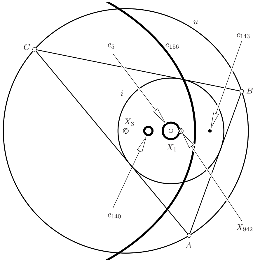
Figure 11: Poristic loci of some nine-point centers: X_5 moves on c_5 . The centers X_{140} and X_{143} are the nine-point centers of \Delta_m and \Delta_o , respectively. According to Theorem 4.6 their poristic loci are the circles c_{140} and c_{143} . The nine-point center of \Delta_t is the point X_{156} . Its poristic orbit is the conic section e_{156} , cf. Theorem 4.7. \Delta 's circumcenter X_3 plays a double-role: It is the nine-point center of \Delta_a and \Delta_e . The nine-point center of \Delta_i is the same point for all triangles in the poristic system, i.e. , X_{942} is fixed, see Theorem 4.1.
