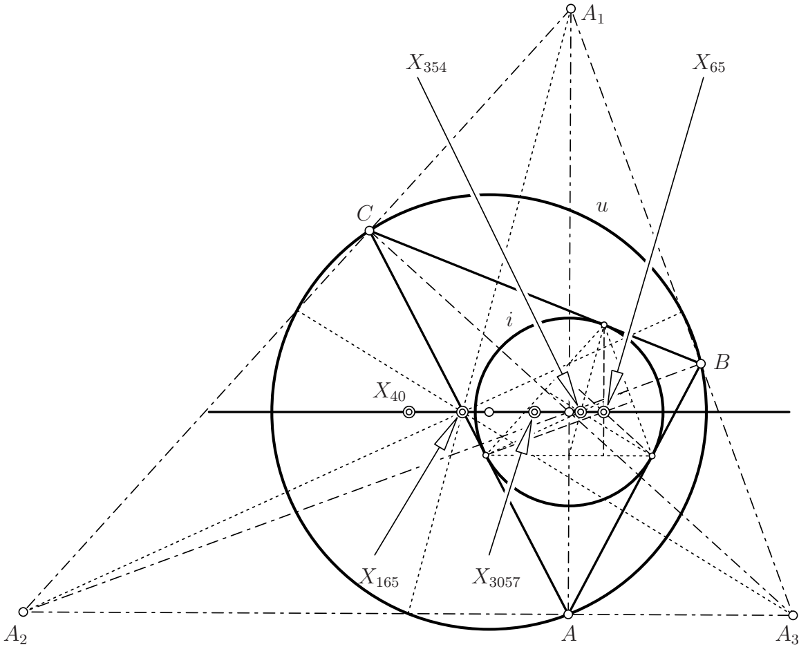
Figure 5: Some centers on the line \mathcal{L}_{1,3} mentioned in Theorem 4.1: the circumcenter X_{40} of \Delta_e , the orthocenter X_{65} of \Delta_i , the centroid X_{165} of \Delta_e , the centroid X_{354} (WEILL point) of \Delta_i , the DE LONGCHAMPS point X_{3057} of \Delta_i .
