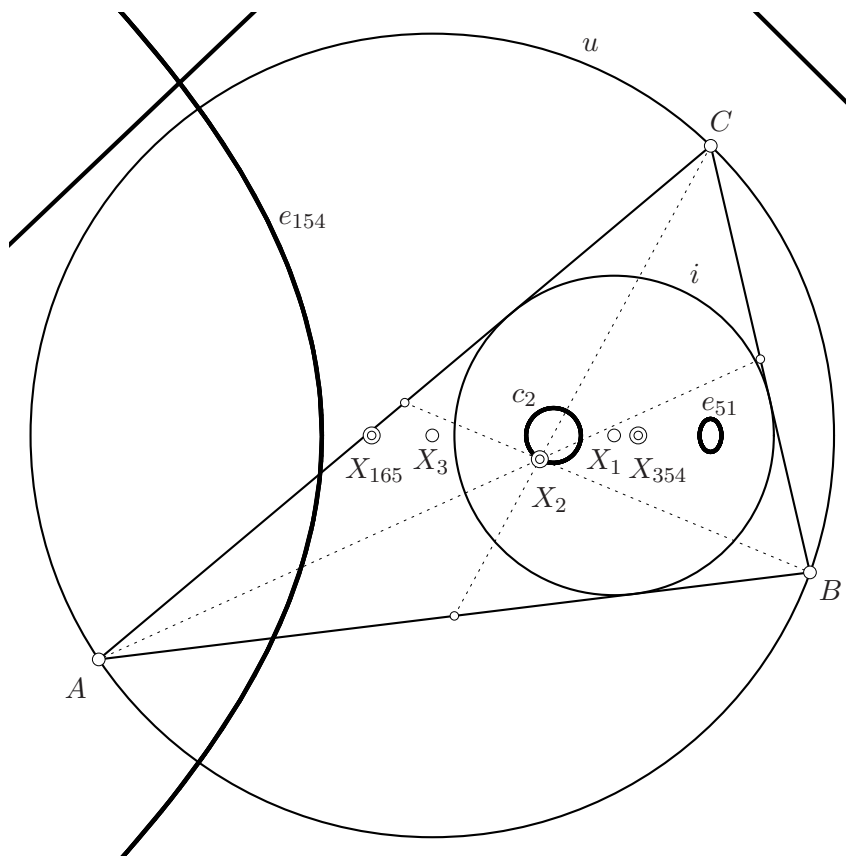
Figure 8: Poristic loci of some centroids: X_2 is the centroid for \Delta , \Delta_a , and \Delta_m at the same time and moves on a circle c_2 , cf. Theorem 4.6. The WEILL point X_{354} (centroid of \Delta_i ) and the centroid X_{165} of \Delta_e remain fixed according to Theorem 4.1. The centroids X_{51} and X_{154} of \Delta_o and \Delta_t , respectively, trace conic sections as stated in Theorem 4.7.
