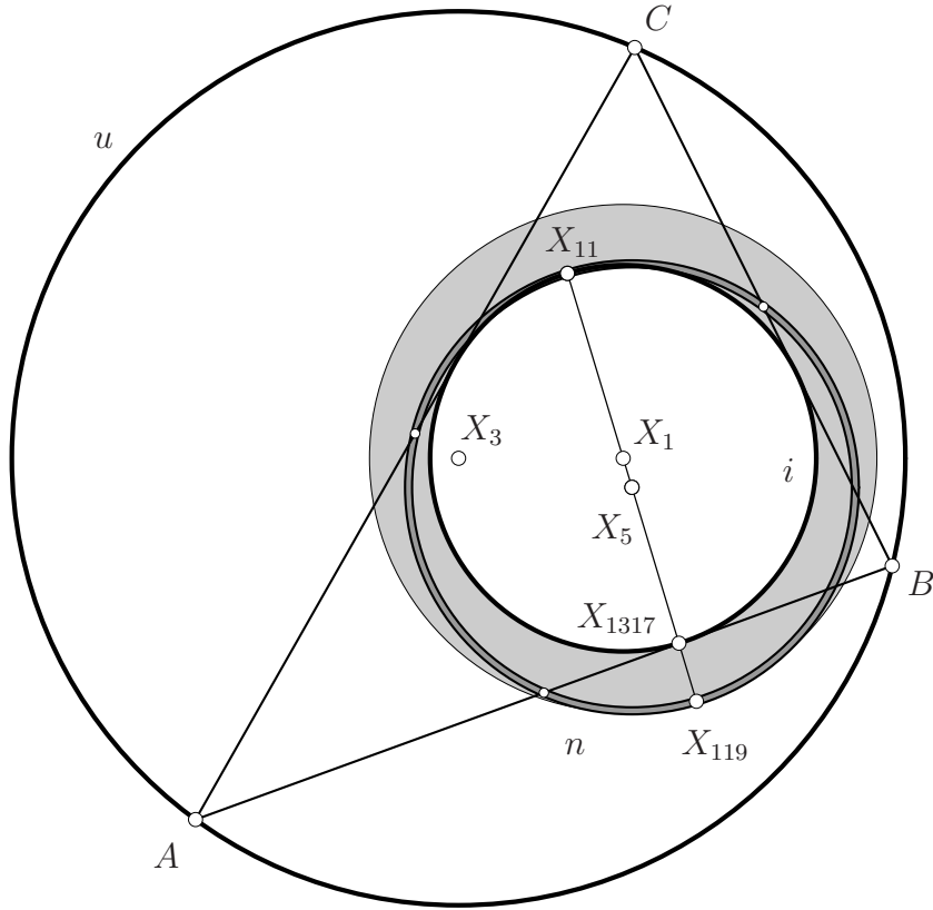
Figure 7: The grey shaded annulus is the locus of all nine-point circles n of triangles in the poristic family
