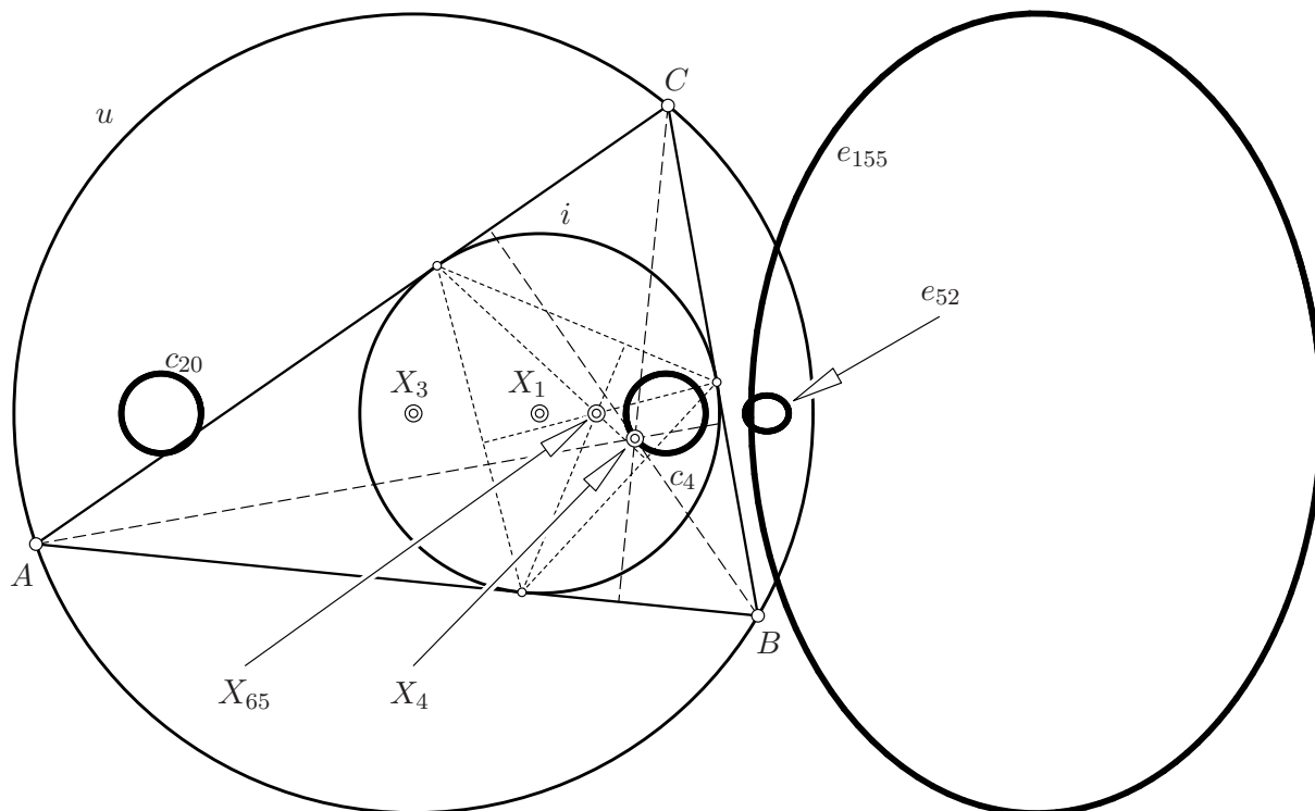
Figure 10: Poristic loci of some orthocenters: \Delta 's orthocenter X_4 circles along c_4 . The DE LONGCHAMPS point X_{20} runs on the circle c_{20} (cf. Theorem 4.6). X_1 , X_3 , and X_{65} are the orthocenter \Delta_e , \Delta_m , and \Delta_i . According to Theorem 3.2 X_{65} remains fixed. The orthocenters X_{52} and X_{155} of \Delta_o and \Delta_t travel along conic sections e_{52} and e_{155} , respectively, cf. Theorem 4.7.
