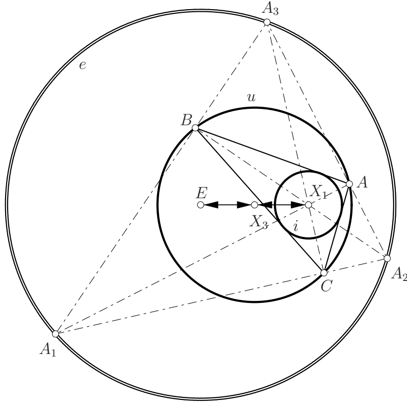
Figure 3: The common path of all three excenters
