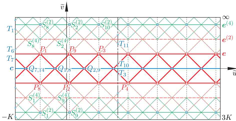
Figure 8: The injective mapping \mathbf{Z} sends the square grid of points Q_i, P_i and S_i^{(j)} , i = 1, 2 \dots, 14 , j = 2, 4 , to the vertices and the diagonals to the net of curvature lines of the Poncelet grid associated to an N -periodic focal billiard on a one-sheeted hyperboloid with N = 14 and turning number \tau = 2 .
