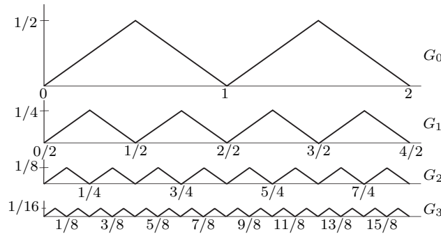
Figure 1.1: The family \{G_n\}
